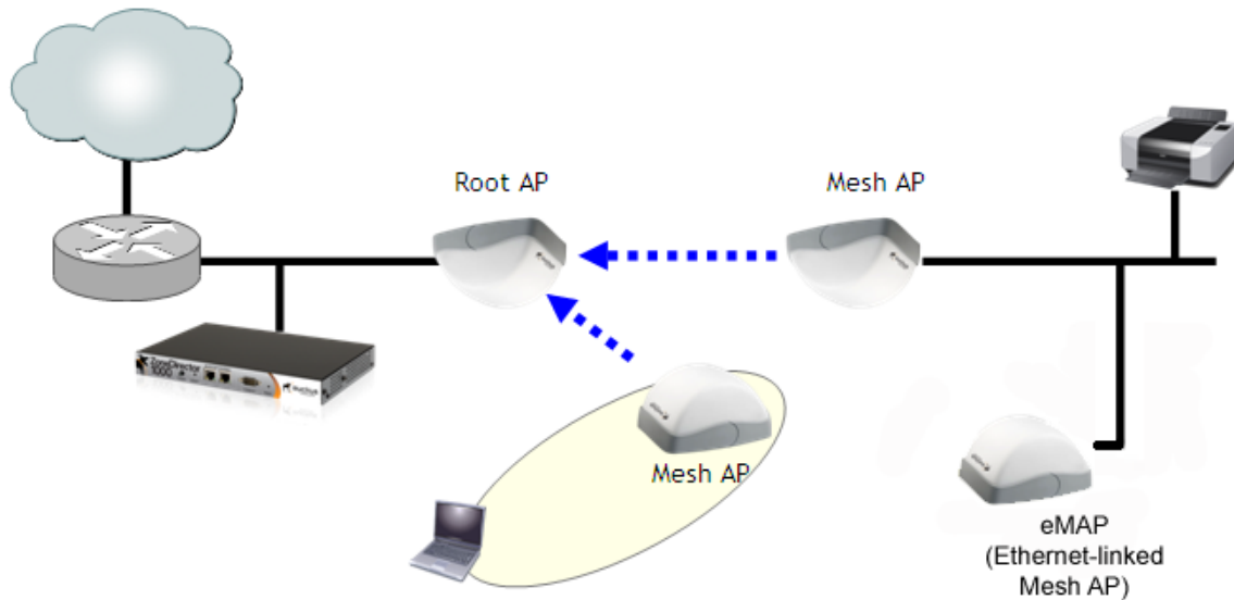
FIGURE 284 eMAP - Hybrid Mesh topology
