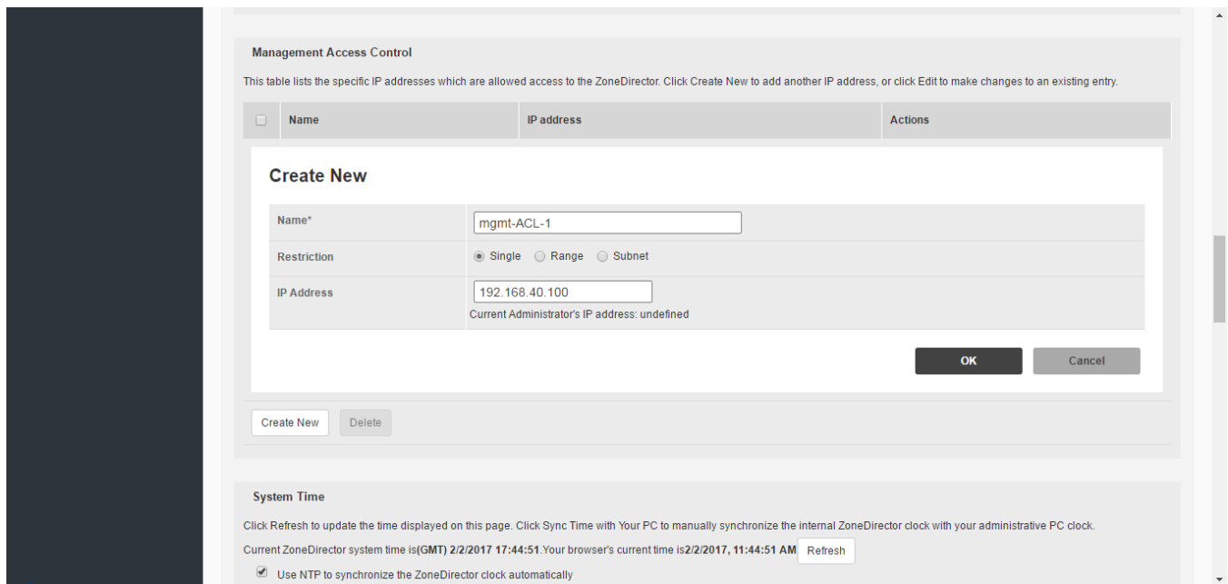
FIGURE 218 Creating a new ZoneDirector management ACL
