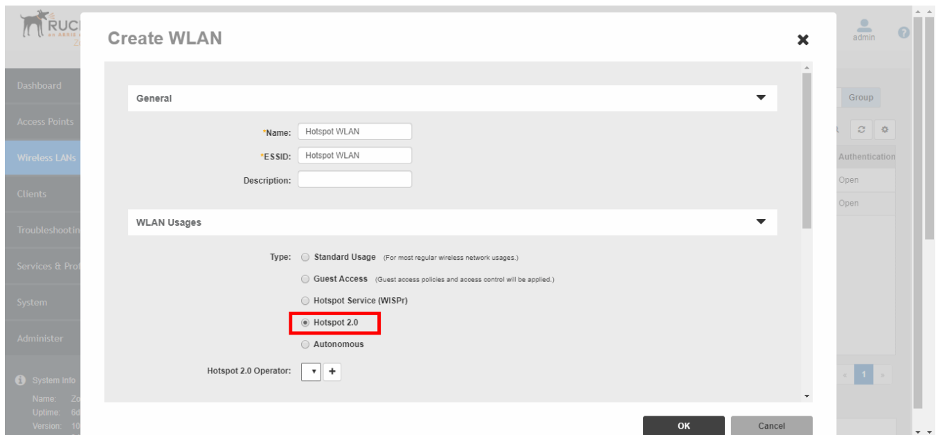
FIGURE 132 Creating a Hotspot 2.0 WLAN
