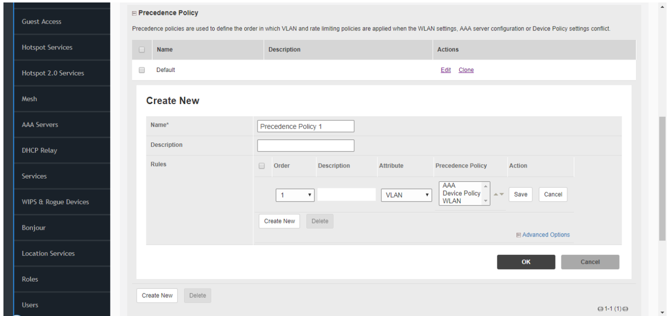
FIGURE 162 Precedence Policy settings
