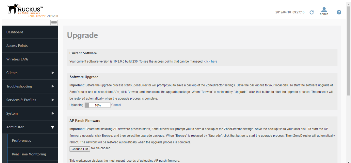
FIGURE 245 Firmware upload in progress
